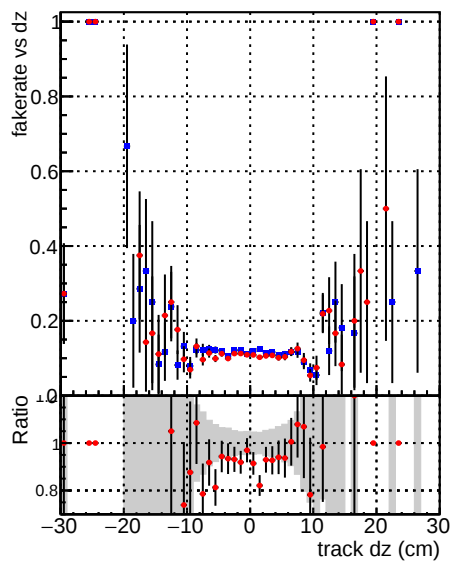
Fake rate vs dz Legend: DQM_mkFit_baseline_lowPT (blue dots) DQM_mkFit_baseline6iter_lowPT (red dots)
