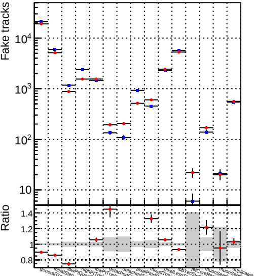
Number —●— DQM_mkFit_TTbase
