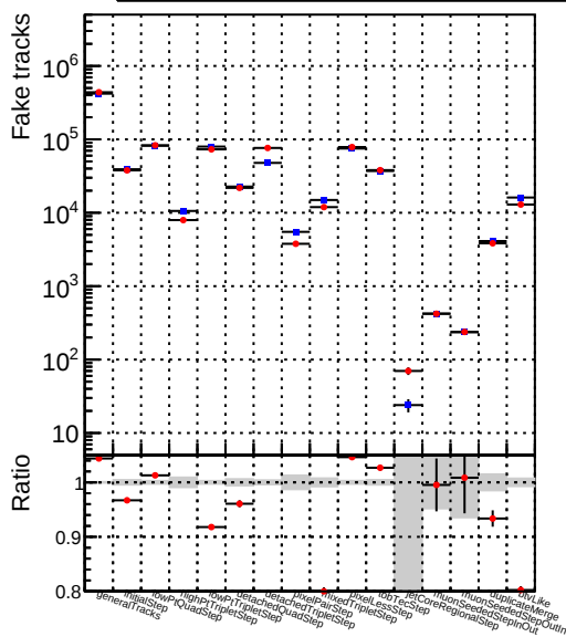
Number —●— DOM mkFit TTbase
