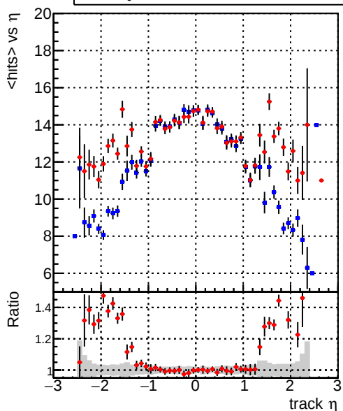
mean hits vs \eta — DQM_CKF_TTbase — DQM_mkFit_TTbase
