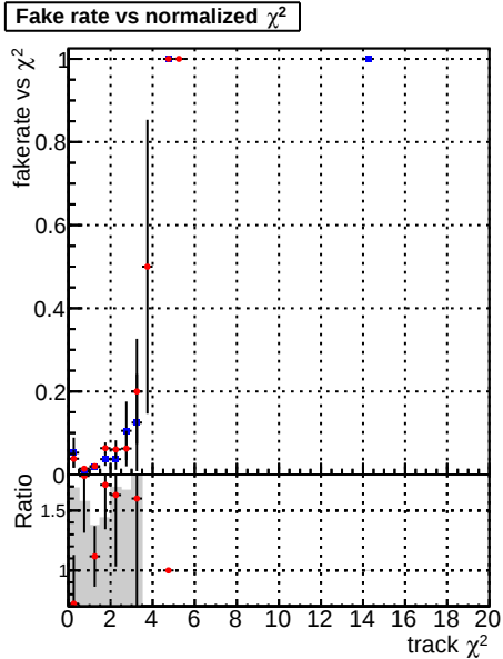
Fake rate vs. █ DQM_CKF_TTbase █ DQM_mkFit_TTbase
