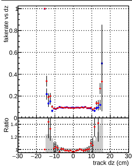
—●— DQM_CKF_TTbase —●— DQM_mkFit_TTbase
