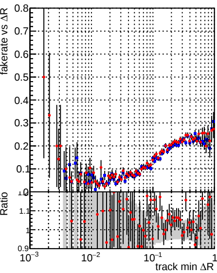
Fake rate vs \Delta R(\text{track, jet}) Legend: \blacksquare DQM_CKF_TTbase \bullet DQM_mkFit_TTbase
