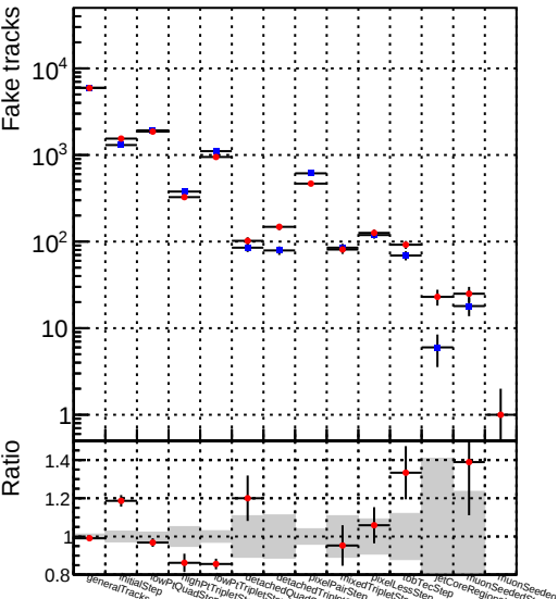
Number —●— DQM_mkFit_TTbase
