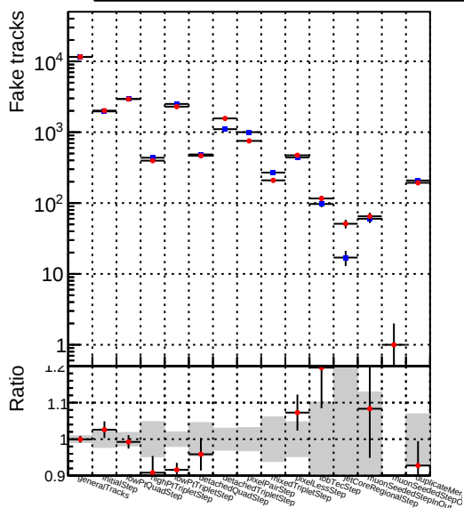
Number —●— DQM_mkFit_TTbase
