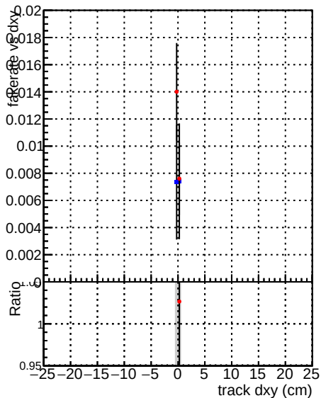
—•— DQM_CKF_TTbase —•— DQM_mkFit_TTbase
