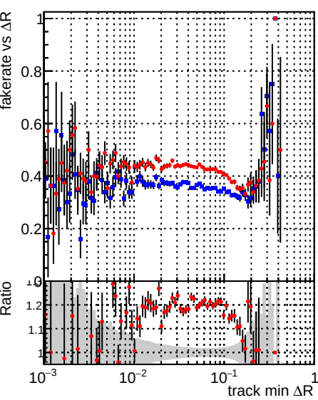
—•— DQM_CKF_TTbase —•— DQM_mkFit_TTbase
