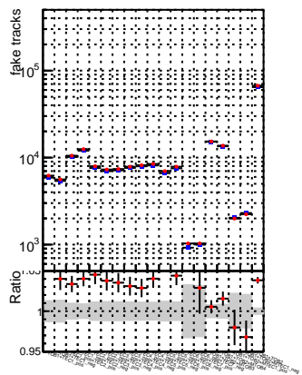
N of associated (recoToSim) fake tracks vs. s
