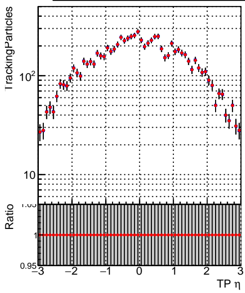
N of simulated tracks vs \eta Legend: DQM_CKF_TTbase (blue line), DQM_mkFit_TTbase (red line)
