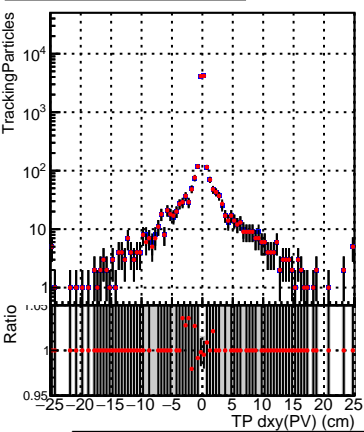
DQM_CKF_TTbase
