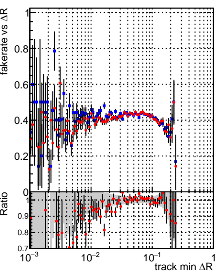
Fake rate vs \Delta R —●— DQM_CKF_TTbase —●— DQM_mkFit_TTbase
