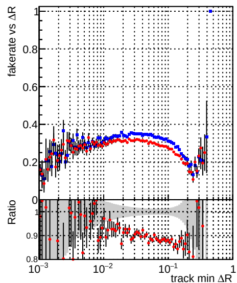
—•— DQM_CKF_TTbase —•— DQM_mkFit_TTbase
