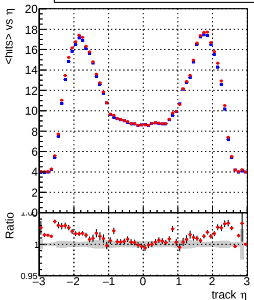
mean hits — DQM_CKF_TTbase — DQM_mkFit_TTbase
