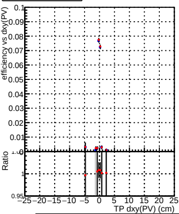
Efficiency vs Dxy(PV) Legend: DQM_mkFit_TT_baseline_6iter (blue squares), DQM_mkFit_TT_RetrainV2_WP1_6iter (red circles)
