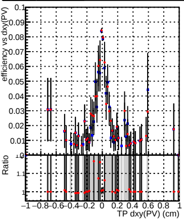
Efficiency vs Dxy(PV) Legend: DQM_mkFit_TT_baseline_6iter (blue squares), DQM_mkFit_TT_RetrainV2_WP1_6iter (red circles)
