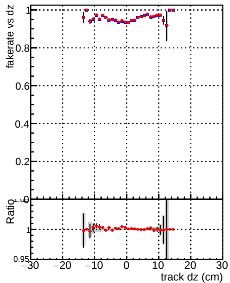
Fake rate vs dz — DQM_mkFit_TT_baseline_6iter — DQM_mkFit_TT_RetrainV2_WP1_6iter
