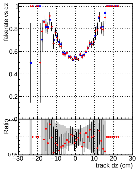
Fake rate vs dz —●— DQM_mkFit_TT_baseline_6titer —●— DQM_mkFit_TT_RetrainV2_WP1_6titer
