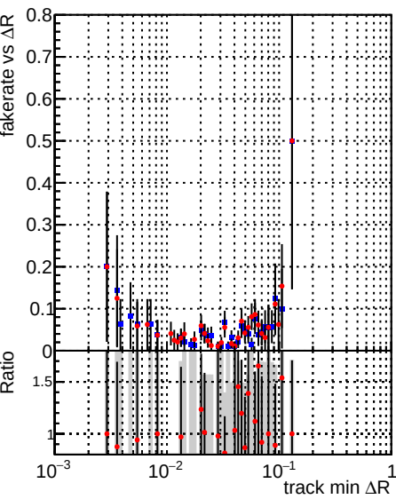
Fake rate vs \Delta R(\text{track, jet}) DQM_mkFit_TT_baseline_6iter DQM_mkFit_TT_RetrainV2_WP1_6iter
