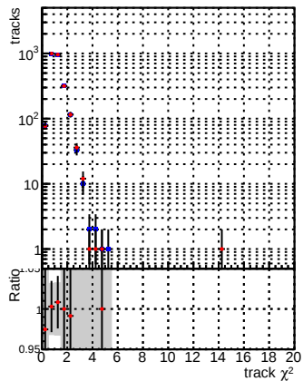
N of reco track vs. \chi^2 for DQM mkFit TT_baseline_6iter and DQM mkFit TT_RetrainV2_WP1_6iter
