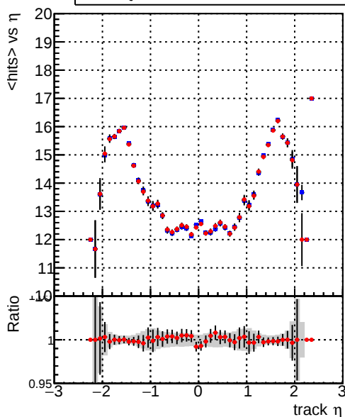
Legend: DQM_mkFit_TT_baseline_6iter (blue line), DQM_mkFit_TT_RetrainV2_WP1_6iter (red line) mean hits vs \eta
