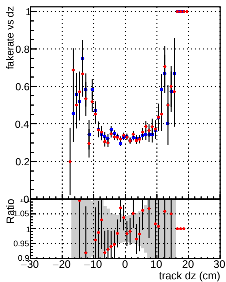
Fake rate vs dz — DQM_mkFit_TT_baseline_6iter — DQM_mkFit_TT_RetrainV2_WP1_6iter
