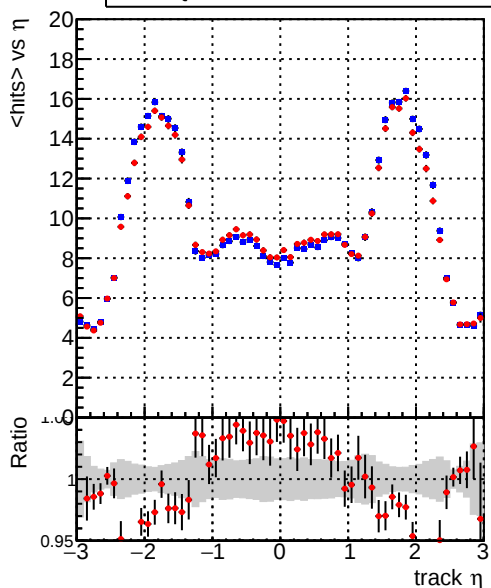
— DQM_mkFit_TT_baseline_6iter — DQM_mkFit_TT_RetrainV2_WP1_6iter mean hits vs \eta
