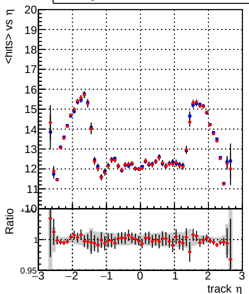
mean hit — DQM_mkFit_TT_baseline_6iter — DQM_mkFit_TT_RetrainV2_WP1_6iter
