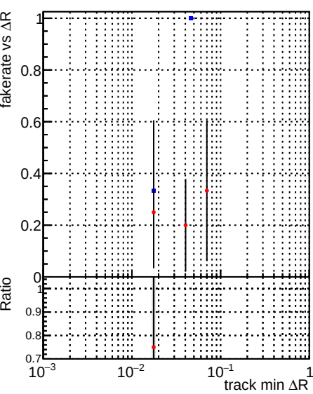
Fake rate vs \Delta R(\text{track, jet}) Legend: DQM_mkFit_TT_baseline_6iter (blue), DQM_mkFit_TT_RetrainV2_WP1_6iter (red)
