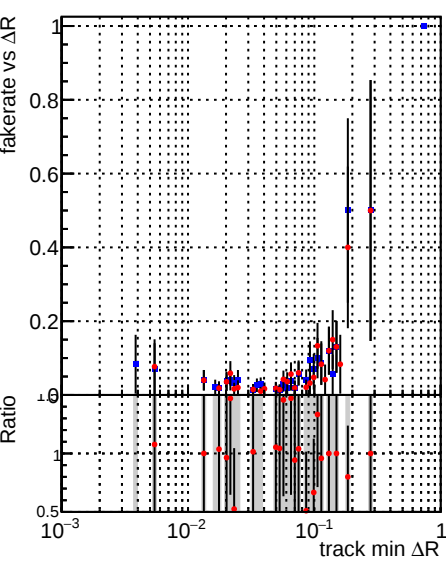
Fake rate vs \Delta R(\text{track, jet}) Legend: —●— DQM_mkFit_TT_baseline_6iter —●— DQM_mkFit_TT_RetrainV2_WP1_6iter
