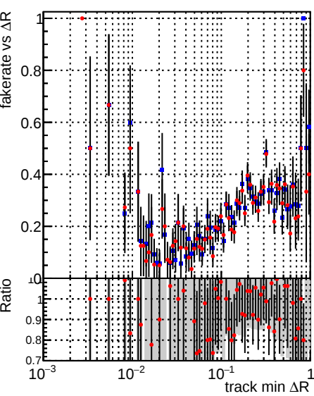
Fake rate vs \Delta R(\text{track, jet}) Legend: DQM_mkFit_TT_baseline_6iter (blue squares) DQM_mkFit_TT_RetrainV2_WP1_6iter (red circles)
