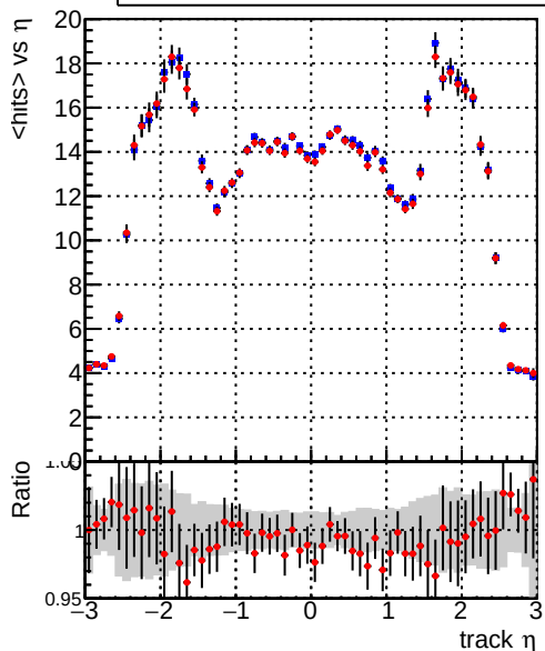
mean hits vs \eta — DQM_mkFit_TT_baseline_6iter — DQM_mkFit_TT_RetrainV2_WP1_6iter
