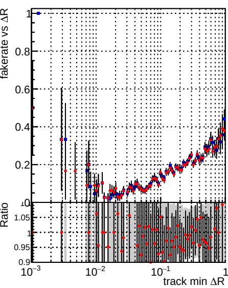
Legend: \blacksquare DQM_mkFit_TT_baseline_6iter \bullet DQM_mkFit_TT_RetrainV2_WP1_6iter
