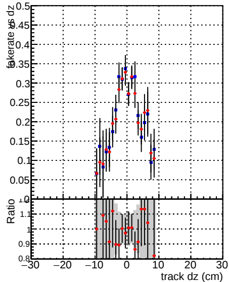
Fake rate vs dz Legend: DQM_mkFit_TT_baseline_6iter (blue dots) DQM_mkFit_TT_RetrainV2_WP1_6iter (red dots)
