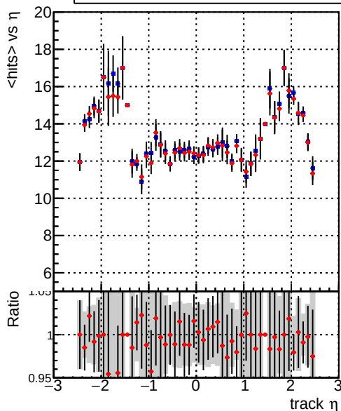
mean hit Legend: DQM_mkFit_TT_baseline_6iter (blue line), DQM_mkFit_TT_RetrainV2_WP1_6iter (red line)
