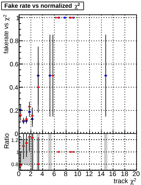
Fake rate vs. Legend: DQM_mkFit_TT_baseline_6iter DQM_mkFit_TT_RetrainV2_WP1_6iter
