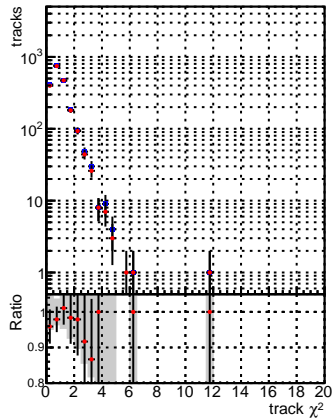
N of reco track vs. \chi^2 —●— DQM_mkFit_TT_baseline_6iter —●— DQM_mkFit_TT_RetrainV2_WP1_6iter
