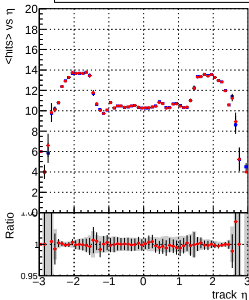
mean hit — DQM_mkFit_TT_baseline_6iter — DQM_mkFit_TT_RetrainV2_WP1_6iter
