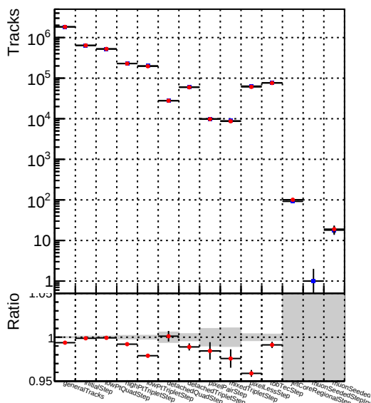
Number of tracks vs collection Legend: DQM_mkFit_TT_baseline_6iter DQM_mkFit_TT_RetrainV2_WP1_6iter
