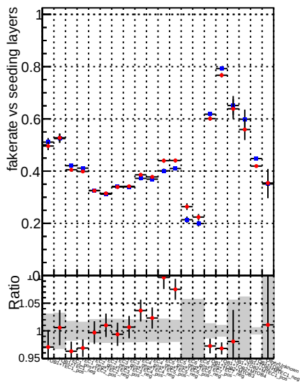
Fake rate vs. — DQM_mkFit_TT_baseline_6iter — DQM_mkFit_TT_RetrainV2_WP1_6iter
