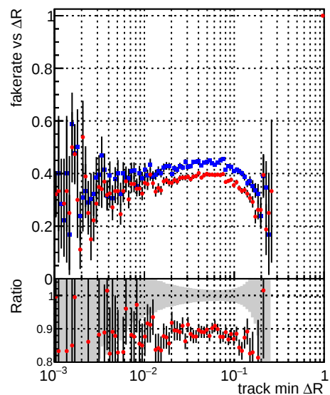
Fake rate vs \Delta R (track, jet) Legend: DQM_mkFit_TT_baseline_6iter (blue line with markers) DQM_mkFit_TT_RetrainV2_WP1_6iter (red line with markers)
