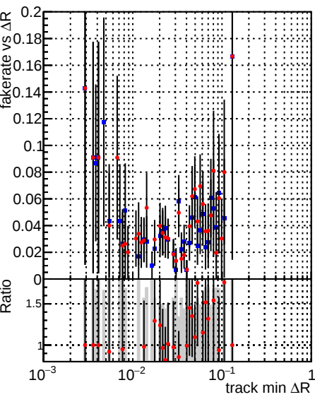
Fake rate vs \Delta R(\text{track, jet}) Legend: \blacksquare DQM_mkFit_TT_baseline_6iter \bullet DQM_mkFit_TT_RetrainV2_WP1_6iter
