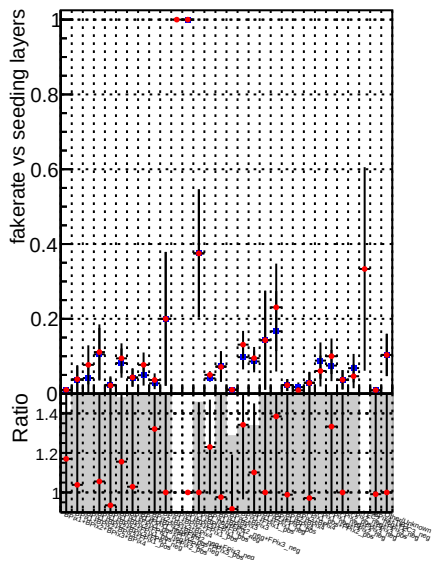
Fake rate vs. — DQM_mkFit_TT_baseline_6iter — DQM_mkFit_TT_RetrainV2_WP1_6iter
