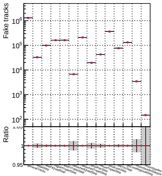
Number 1 DQM_CKF_TT_baseT125_noSel
