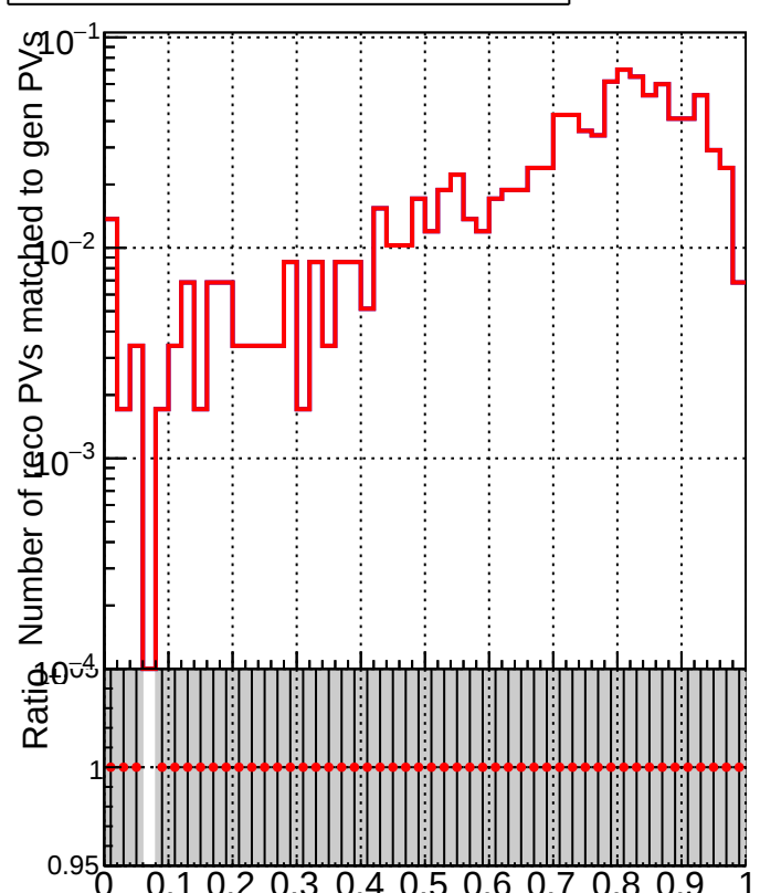
RecoPVAssoc2GenPVMatched_missing
