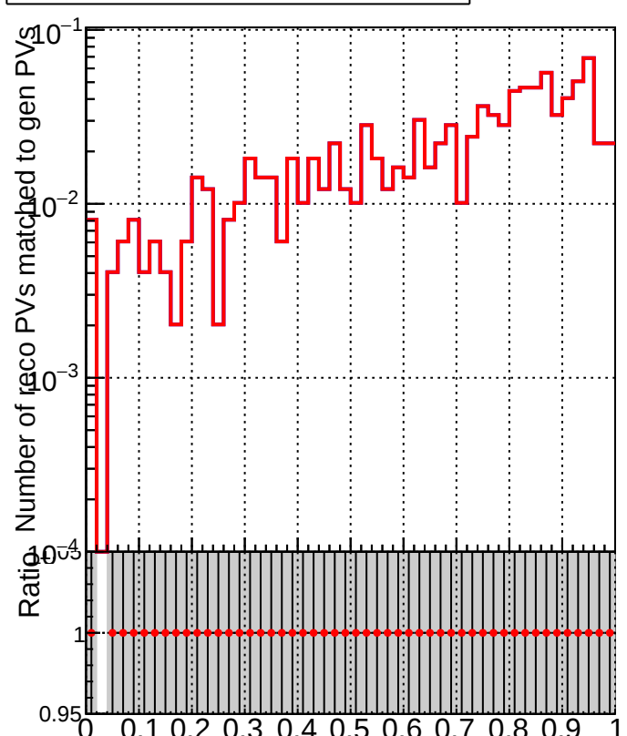
RecoPVAssoc2GenPVMatched_Purity
