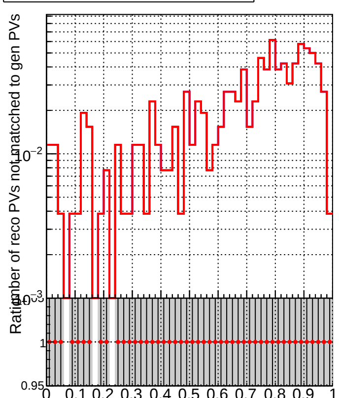
RecoPVAssoc2GenPVNotMatched_missing
