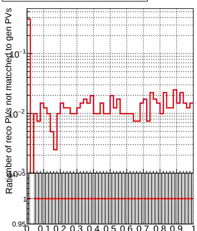
RecoPVAssoc2GenPVNotMatched_Purity
