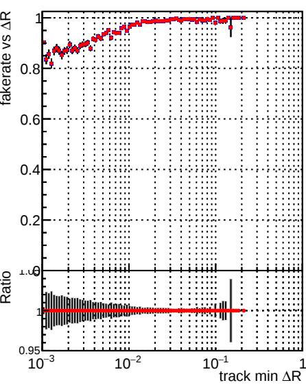
Legend: \blacksquare DQM_CKF_TT_base_noSel \bullet DQM_CKF_TT_baseT125_noSel
