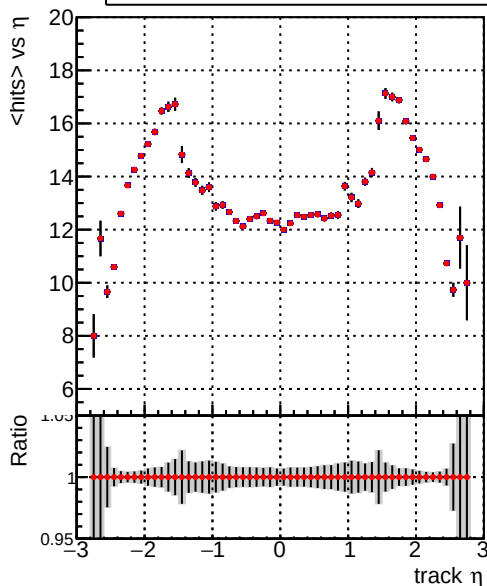
mean hits — DQM_CKF_TT_base_noSel — DQM_CKF_TT_baseT125_noSel
