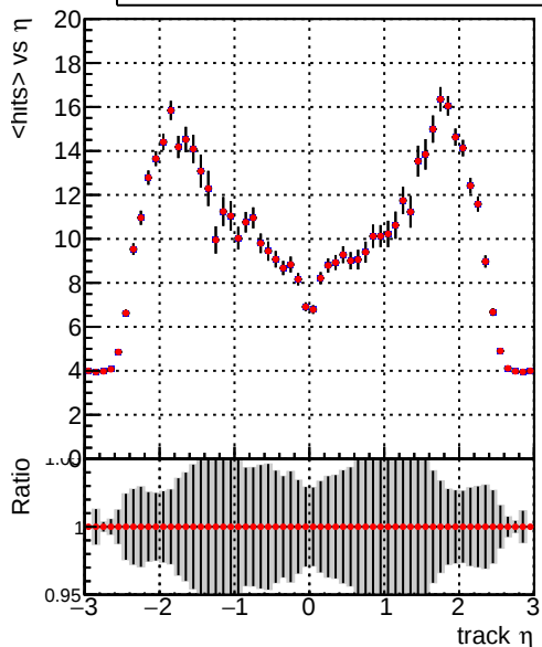
mean hit — DQM_CKF_TT_base_noSel — DQM_CKF_TT_baseT125_noSel
