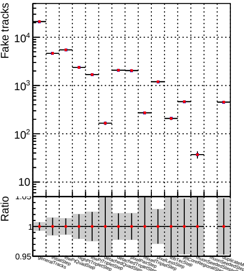
Number —●— DQM_CKF_TT_baseT125_noSel
