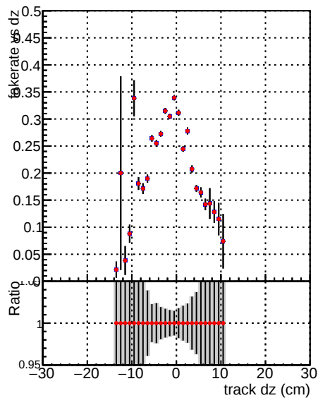
Fake rate vs dz —●— DQM CKF TT_base noSel —●— DQM CKF TT_baseT125 noSel
