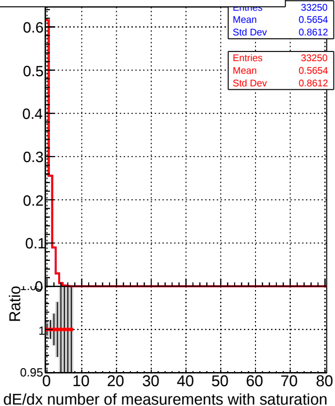
█ DQM_CKF_TT_base_noSel —●— DQM_CKF_TT_baseT125_noSel
