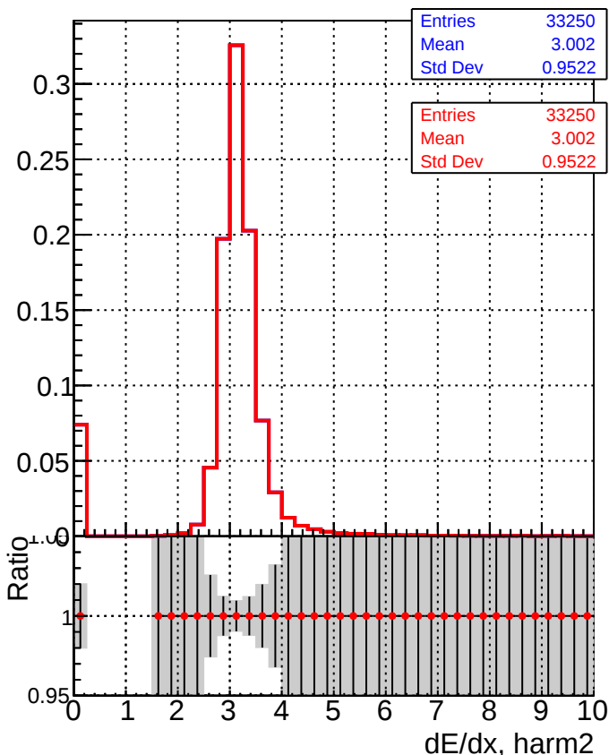
█ DQM_CKF_TT_base_noSel —●— DQM_CKF_TT_baseT125_noSel
