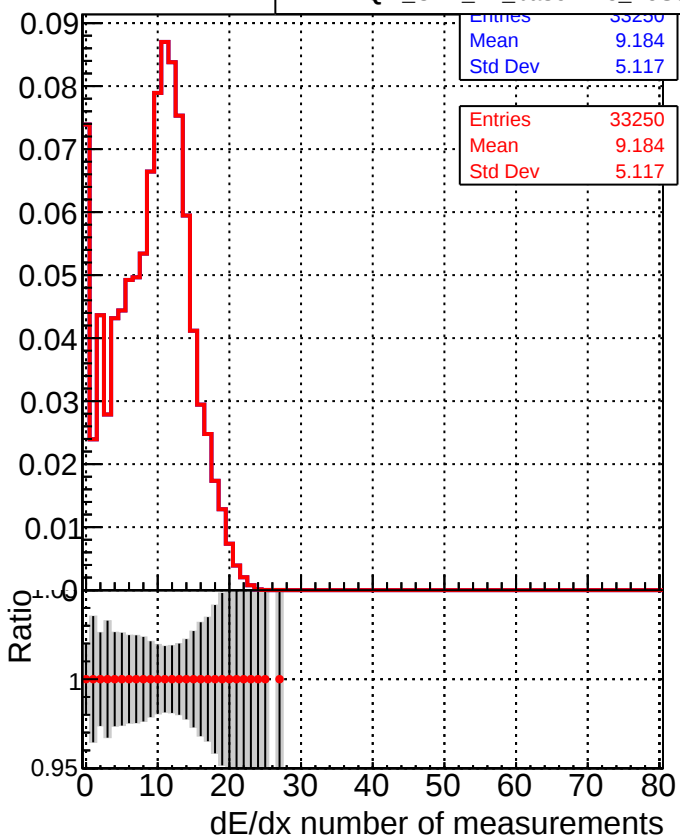
█ DQM_CKF_TT_base_noSel —●— DQM_CKF_TT_baseT125_noSel
