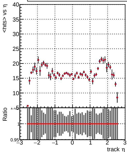
mean hits vs \eta — DQM_CKF_TT_base_noSel — DQM_CKF_TT_baseT125_noSel
